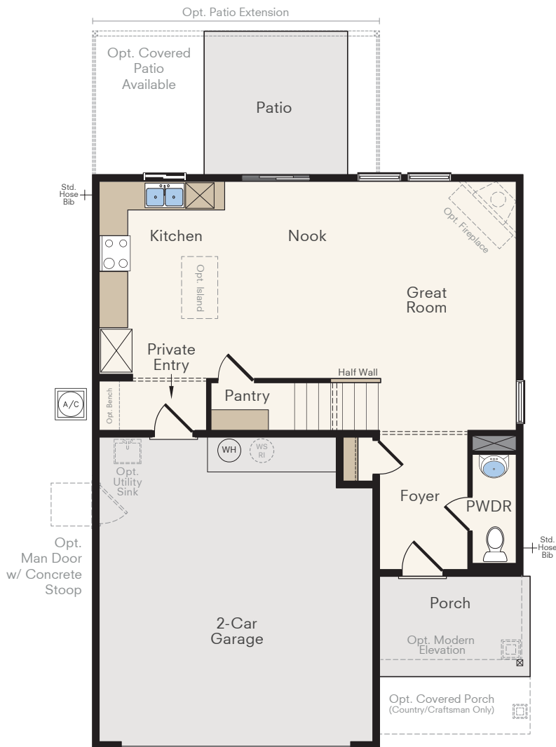
First Floor
